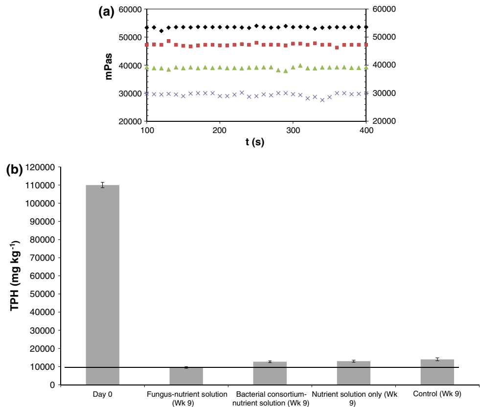
Fig. 1 Changes in oil viscosity (a) and soil TPH levels in laboratory-based microcosms (b). Note For (a), cross symbol, triangle, square and diamond refer to microcosms with fungus, bacterial consortium, control at day 7 and control at day 0, respectively
